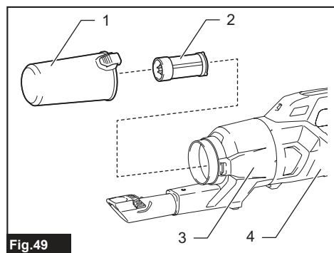
► 1. Dust case 2. Mesh filter 3. Cyclone body 4. Cleaner body
