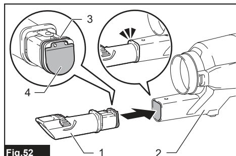
► 1. Inlet pipe 2. Cyclone body 3. O-ring 4. Flap valve
