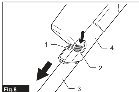
► 1. Release button 2. Arm of release button 3. Attachment with lock function 4. Suction inlet
