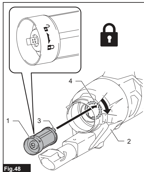
► 1. Mesh filter 2. Cyclone body 3. Hook 4. Port
