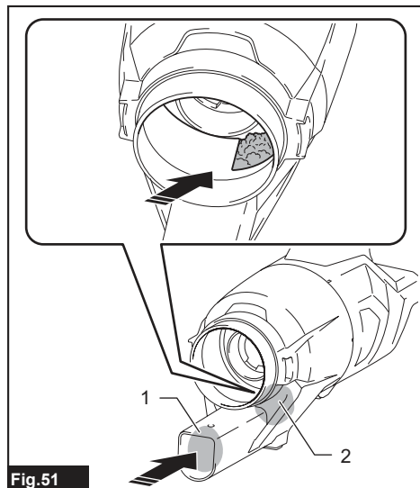
► 1. Suction inlet 2. Incoming air port
