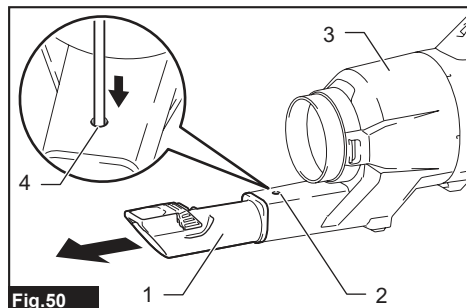
► 1. Inlet pipe 2. Guide stopper 3. Cyclone body 4. Locking hole
